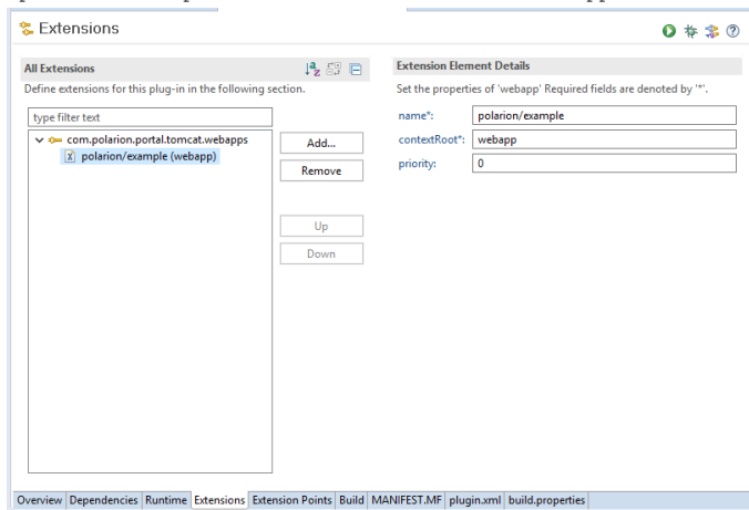
Figure SE-6: Extensions page
