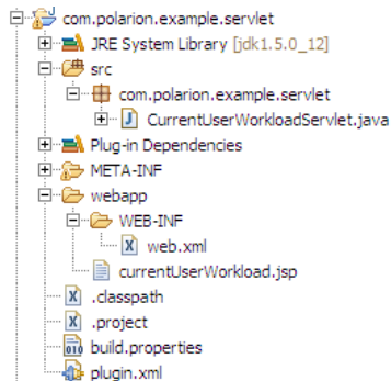
Figure SE-8: Projects files and directories
