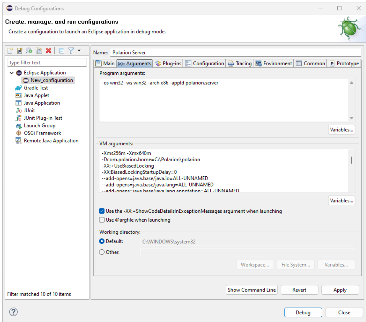
Figure EXEC-2: Debug - Arguments page
