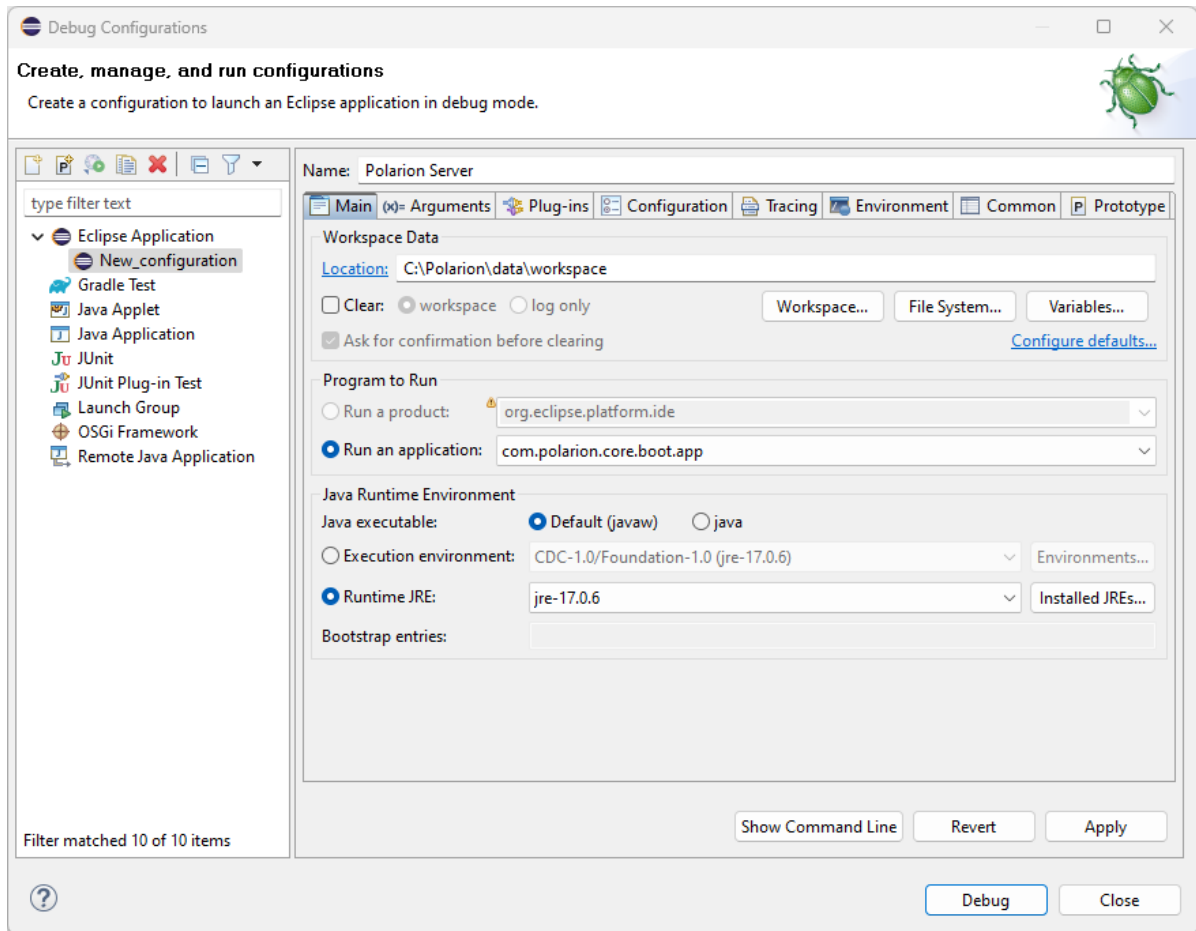
Figure EXEC-1: Debug - Main page
